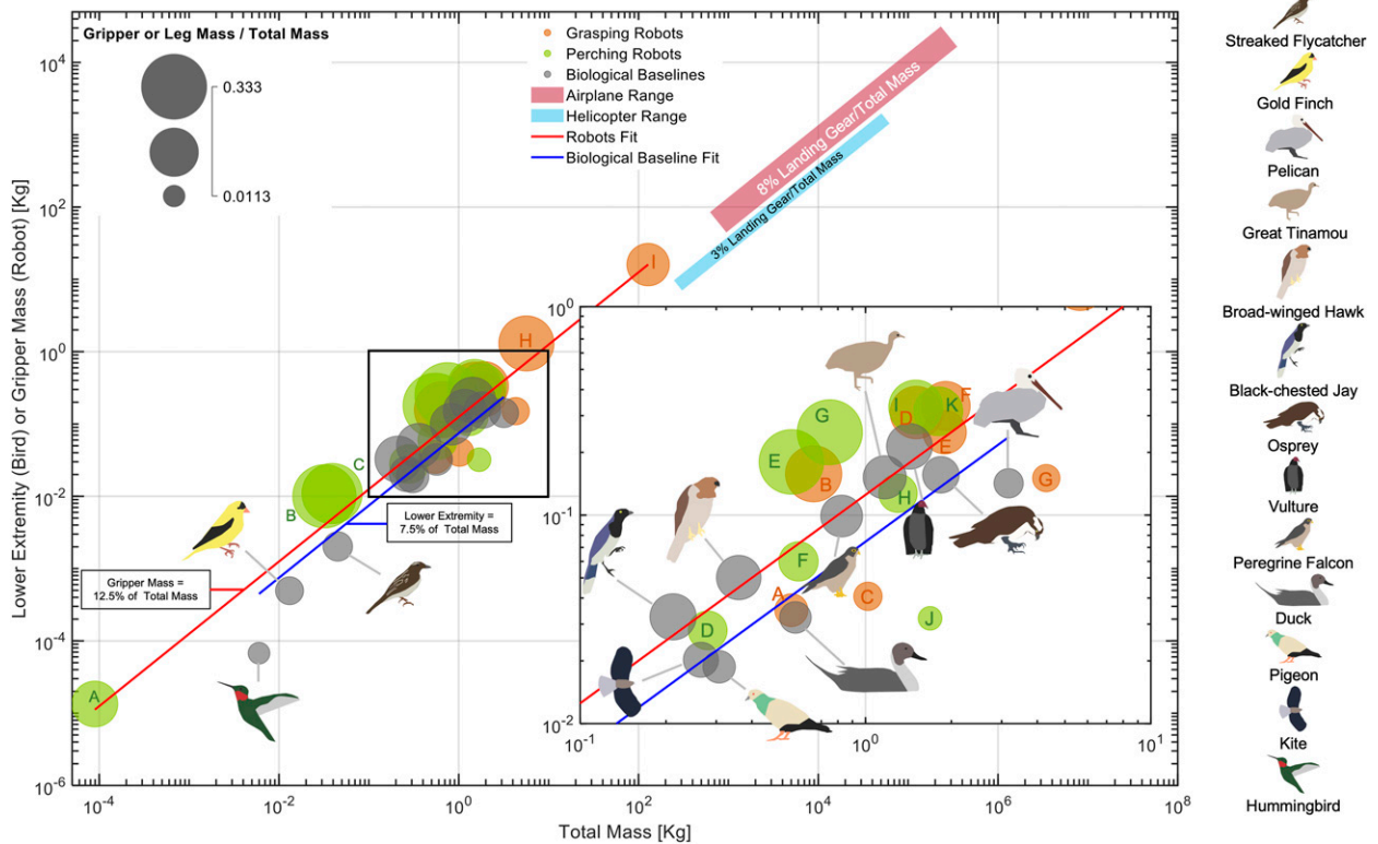
Figure 10. Grasping and perching robots consistently allocate more of their mass towards their manipulators relative to the lower extremities of their avian biological counterparts. This figure shows a comparison of leg or gripper mass as a proportion of total mass of robots and birds across varying mass scales. Biological baselines are included to provide context for the robot prototypes. Letters in circles correspond to robot details in Table 3. All data and sources available in Table 3.
