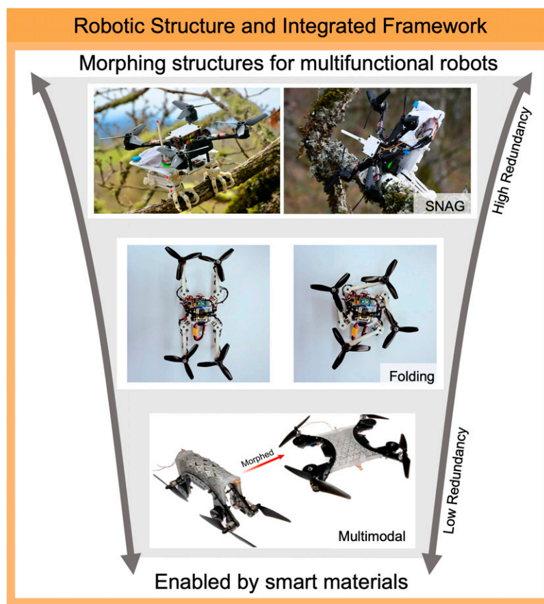
Figure 6. Morphing structural materials will enable adaptability, new use cases, and better environmental resilience. Variable stiffness morphing materials support multifunctional structures to enable multimodal robots and while reducing overengineering and redundancy. 2,132,133
