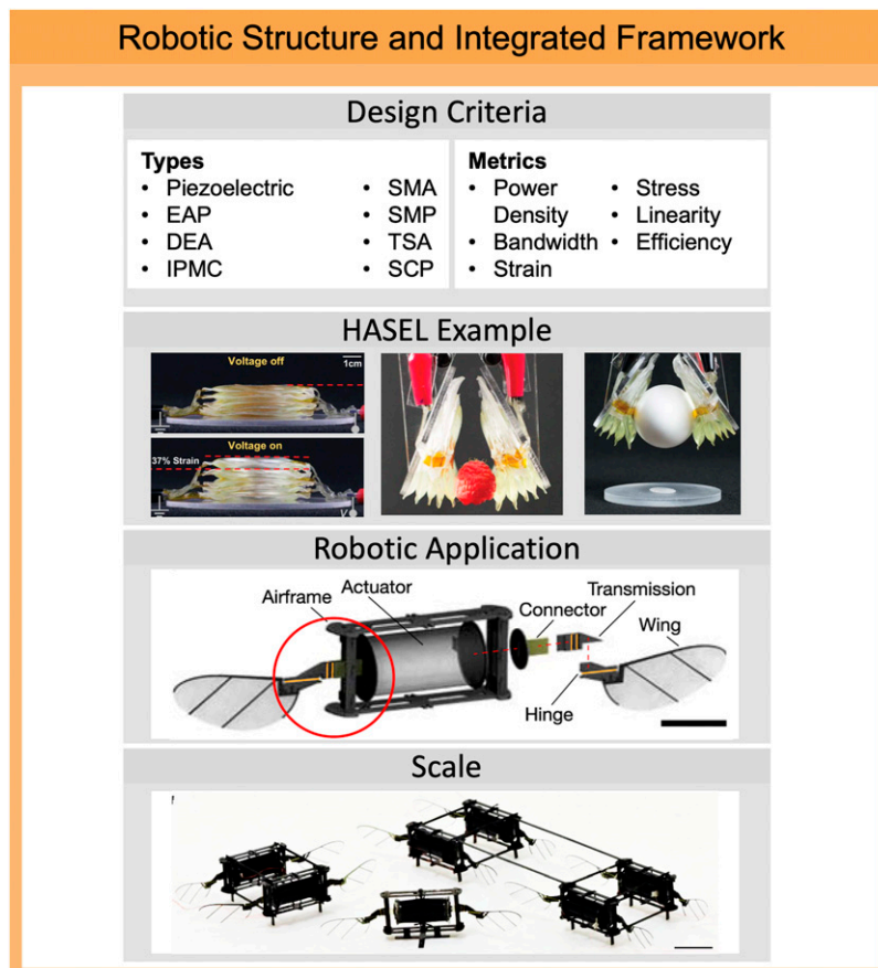
Figure 7. Robotic artificial muscles are a promising technology to replace complex motor and servo driver mechanisms with more forgiving soft actuators. 142 These artificial muscles are typically in one of eight categories and are evaluated using six different performance metrics. 142 A leading example is HASEL. 143 Artificial muscles have been applied to scalable small flapping robots. 144 Applying these technologies could improve SNAG’s performance, decrease repetitive structures used in its design, and reduce assembly complexity.
