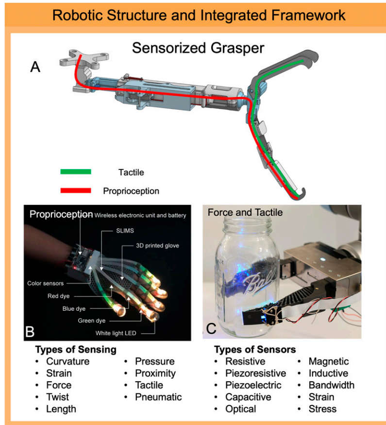
Figure 11. To perceive their environments and the target, grippers must be sensorized. Smart materials can be used for local proprioception, force, and tactile sensing. (A) The ideal regions for the two desired types of sensing are depicted by the colored lines and include proprioception and tactile sensing. (B) A soft skin for human hands demonstrates optical based proprioception. 169 (C) A compliant gripper (GelSight Fin Ray) with GelSight finger tips can infer forces and detect touch using optical sensing. 170 [Bottom Row] Types of sensing and sensors typically used in soft robotic grippers. 168,171
