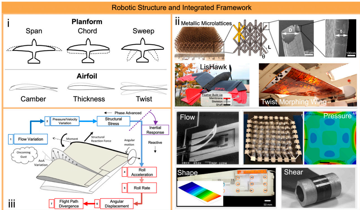
Figure 4. Morphing wings with embedded actuation and sensing can improve flight performance, control, and environmental resilience. (A) The two main categories of wing morphing are airfoil and planform morphing. 68 In airfoil morphing, the shape of the airfoil changes in the plane, in planform morphing the overall shape of the wing changes. 68 (B) New materials for wing morphing include embedded actuation and hierarchical materials that replicate the behavior of biomaterials. Smart materials are relevant at both the wing structure level as well as the wing material level. The “twist morphing wing” uses structures with different material and structural stiffnesses to demonstrate active continuous wing twisting 69 [Photo Credit Kenneth Cheung/NASA]. LisHawk 26 flies with morphing wings and tails buildup by artificial feathers. Metallic micro-lattices are one promising hierarchical material which could be used to develop new wing structures and surfaces. 70 The bottom half of the panel shows different types of embedded wing sensors, including flow, 71 pressure, 72 shape, 73,74 and shear 75 sensing. Pressure and shear sensing enable fly-by-feel, which is based on wrench (force and torque feedback) control to improve flight performance. Shape sensing could be used in vision based autonomous aerial robots for active camera calibration. Shear, pressure and flow sensing can be used to detect flow separation and laminar-turbulent boundary layer transition to optimize wing aerodynamics. (C) Traditional aerial robots have IMUs embedded that are reactive sensors that measure changes in magnetic heading, angular rates and linear acceleration. 76 Phase-advanced sensors measure or predict a disturbance before an inertial response. Embedded sensing in the wings enables an aerial robot to respond to aerodynamic disturbances and compensate for them in advance of the inertial response of the whole vehicle.
