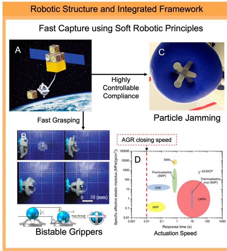
Figure 12. For optimal aerial grasping, the gripper must be fast closing and able to dampen impacts. Smart materials can be integrated to incorporate fast and compliant grasping mechanisms. Two soft robotic principles should drive material development for aerial grasping robots. Future materials should be fast and highly controllable, compliant materials. (A) A proposed fast capture mission in space. 179 (B) A bistable gripper that can close quickly and conform to a variety of object shapes. The top set of images are a time sequence of the gripper actuating and the bottom set are a similar CAD sequence of the gripper activating. 179 (C) A particle jamming gripper with high variable compliance, extreme conformability, and high grasping forces. 180 (D) A plot of the response times of existing materials used in soft robotic grippers. 135
