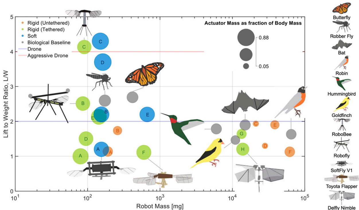
Figure 8. A case study in applying soft acutators to aerial robots. A comparison of existing flapping robots with both artificial muscles and rigid actuators. Biological baselines are included to give context for the robotic prototypes. All muscle actuator robots are tethered during flight. Data and sources available in Table 2.
