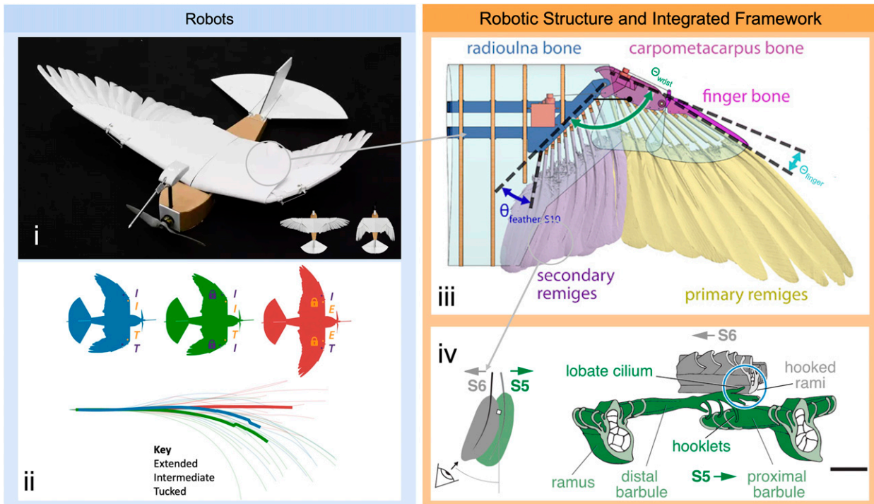
Figure 3. PigeonBot uses an underactuated soft robotic wing with real feathers from a pigeon to stably control its flight. 9 (A) An overview of the aerial robot that demonstrates the ability to morph by changing the planform's shape. The two small images in the bottom right show the extension and flexion range of the morphing wing. (B) A subset of the curved trajectories initiated through asymmetrical wing morphing, showing the robot can turn by morphing one wing half more than the other. (C) A CAD model of the morphing wing design shows how real bird secondary and primary flight feathers are integrated in the biohybrid design. The feathers are mounted on feather holders that connect via a pin joint with the 3D printed bone structure. The bone structure features a servo-actuated wrist and finger joint that form biomimetic robot arms. The feathers are connected by tuned elastic bands (not shown) that mimic the avian elastic ligament that automatically coordinates feather motion when the robot arms move. The ability of feathers to overlap smoothly stems from their graded softness and enables the robot to morph continuously in flight. (D) Adjacent flight feathers have contact zones that match and lock together probabilistically when feathers spread apart too far, and unlock again automatically when they fold together again, making the fastening mechanism directional. 20 The upper surface of the underlapping feather has thousands of 3D hooked lobate cilia (of about 10 micron size) that latch onto the 2D hooked rami that stick out from the lower surface of the overlapping feather. 20
